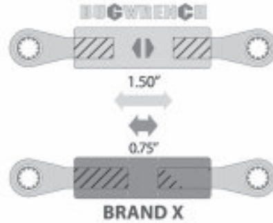
Twice the Metal-to-Metal Electrical Isolation 9/16" x 3/4" model data
